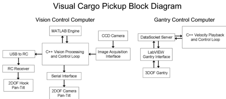
Figure 2. GANTRY CONTROL SYSTEM BLOCK DIAGRAMS
