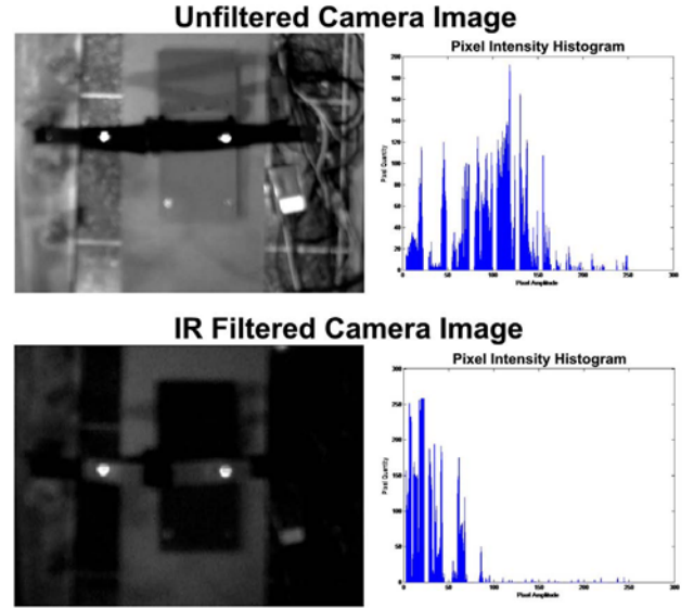
Figure 3. EFFECT OF IR FILTER ON ACQUIRED IMAGES
