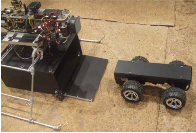
Figure 5. SR-100 WITH CARGO BAY AND UGV
