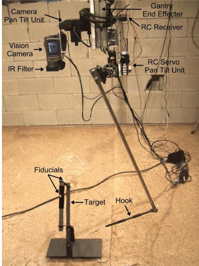
Figure 1. CARGO PICKUP PROTOTYPE
