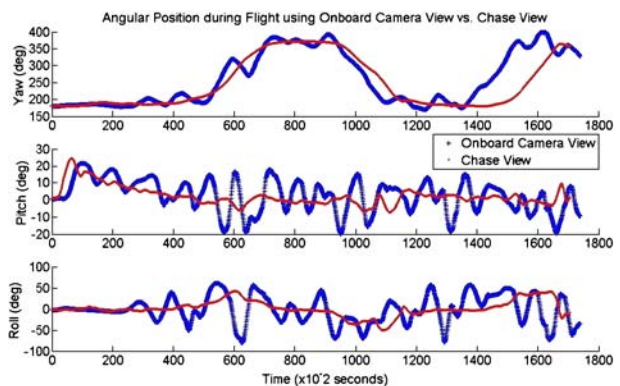
Fig. 12 Example data of the aircraft angular positions during an onboard camera and chase view test. The thicker line represents angles achieved using the onboard camera view the thinner line represents the angles achieved using the chase view
